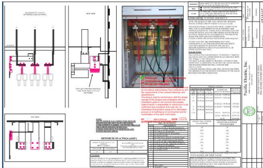
New Incoming PV Power Tap Connection Design
