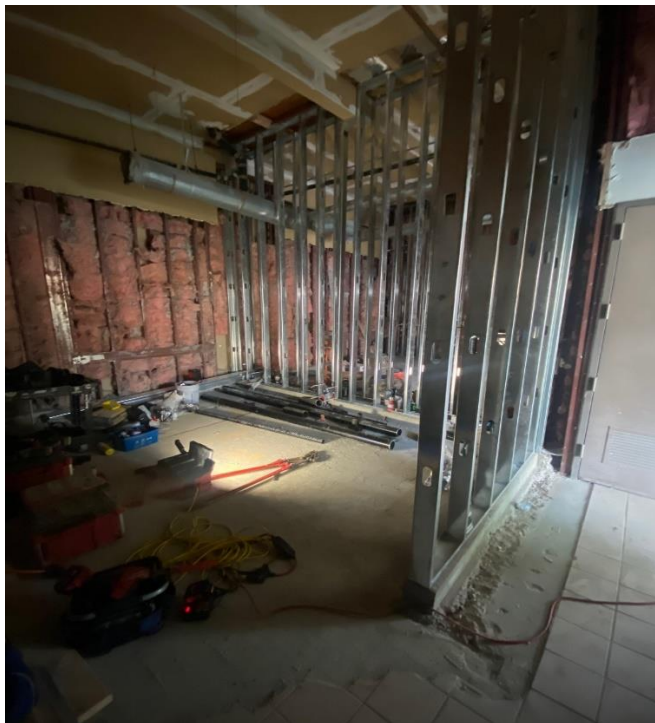
A200 Restroom – Installation of Metal Stud Framing and Plumbing Sanitary Pipe Work
