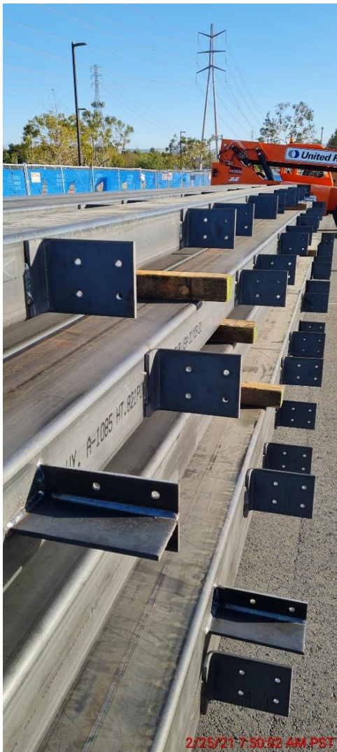
Purlins on Site
