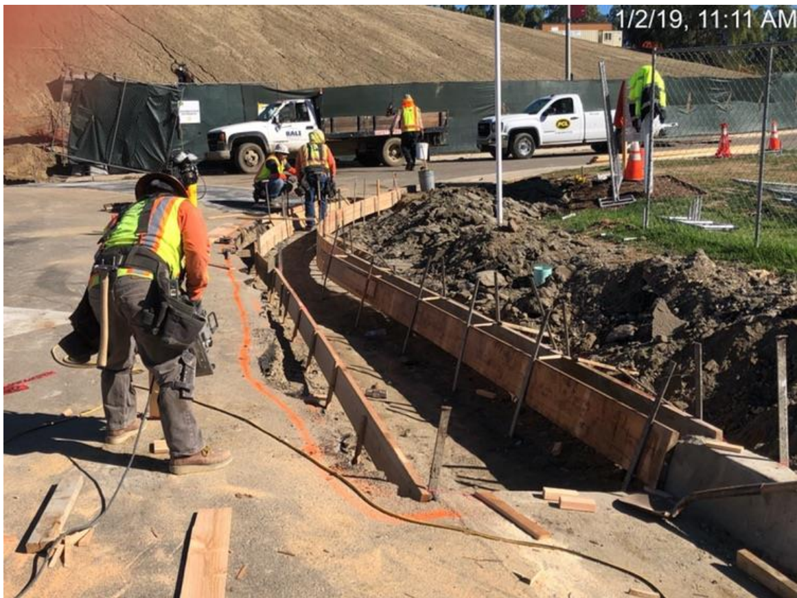
Contractor Preparing Concrete Pour for New Sidewalk at Avery Intersection at Storm Drain Tie-in
